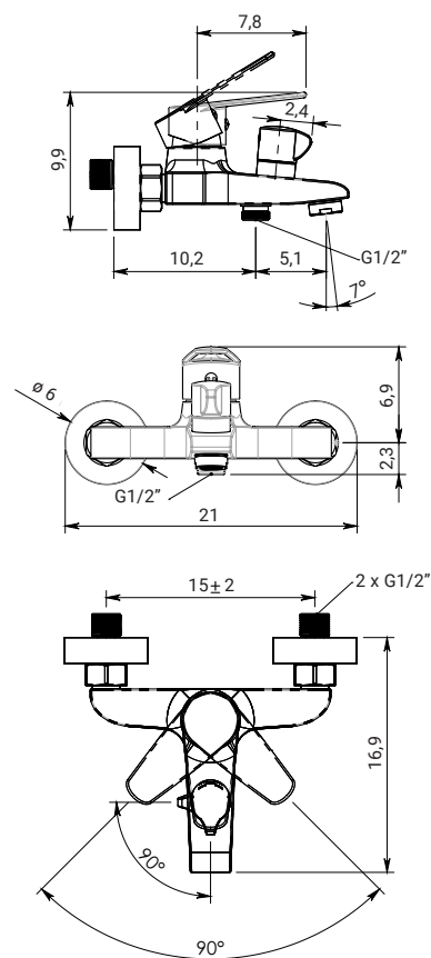
Miscelatore vasca Bathtub mixer
