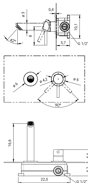
Miscelatore lavabo da muro Wall-mounted washbasin mixer
